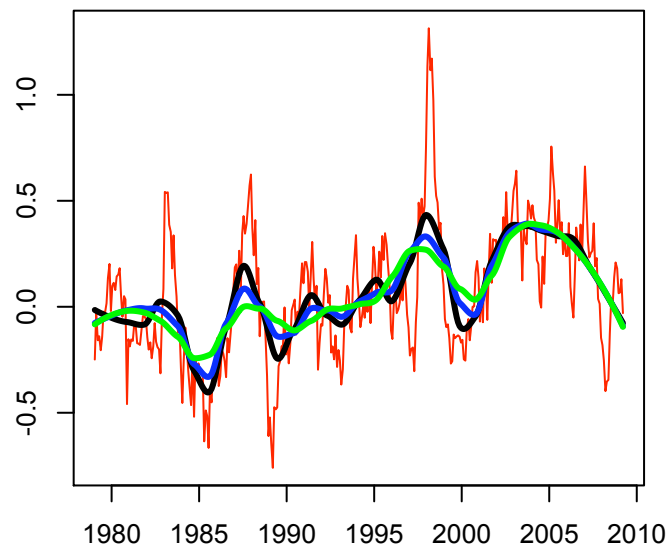
RSS Tropics Temp
