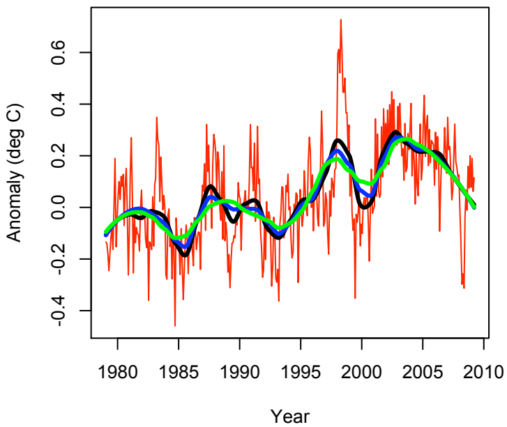
RSS Southern Hemisphere Temp
