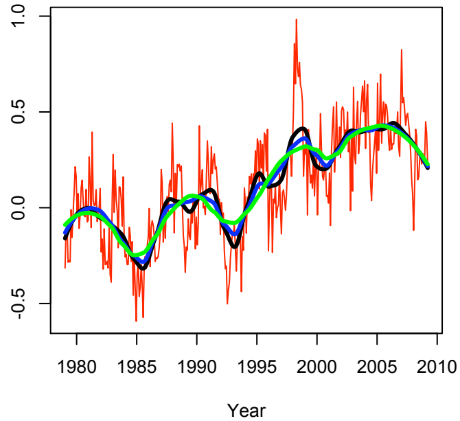
RSS Northern Hemisphere Temp
